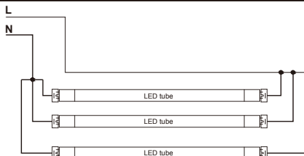
3 LED Tube
