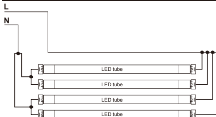
4 LED Tube
