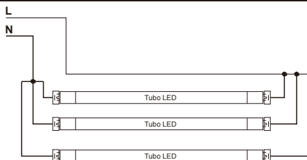
Tubo LED 3
