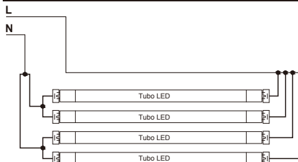
Tubo LED 4
