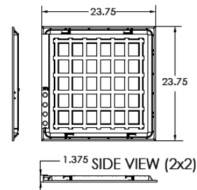
TOP VIEW (2x2)
