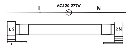
RETROFIT LUMINAIRE WITH 1 LAMP
