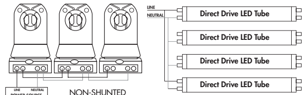
Single Ended Wiring
