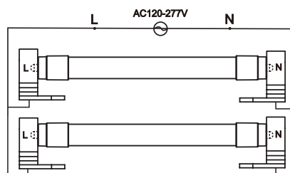
RETROFIT LUMINAIRE WITH 2 LAMPS
