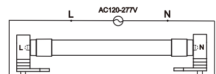
RETROFIT LUMINAIRE MAGNETIC BALLAST
