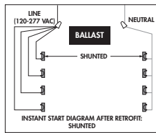
Double Ended Wiring
