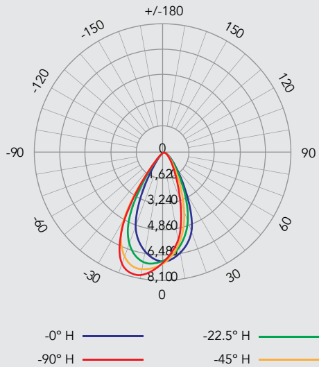
LUMINOUS INTENSITY DISTRIBUTION (4 FT STRIP)
