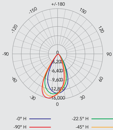
LUMINOUS INTENSITY DISTRIBUTION (8 FT STRIP)
