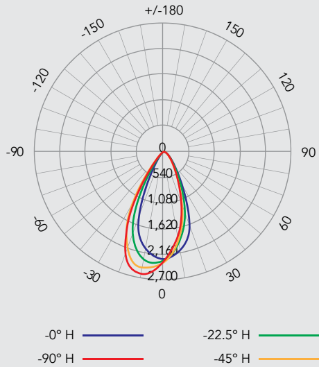
LUMINOUS INTENSITY DISTRIBUTION (2 FT STRIP)
