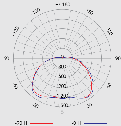
HALO URBAN POST TOP (45W@3000K)
