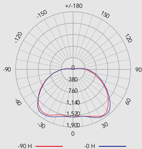
HALO URBAN POST TOP (60W@3000K)
