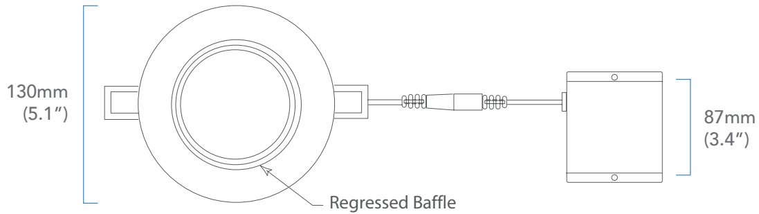
4" Regress Downlight with Baffle
