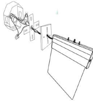
Flag Mount
