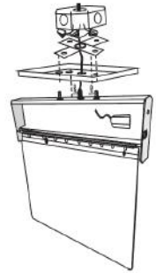
Ceiling Mount
