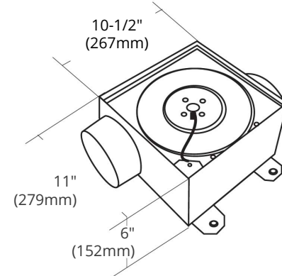
SDF200 Dimensions Diagram
