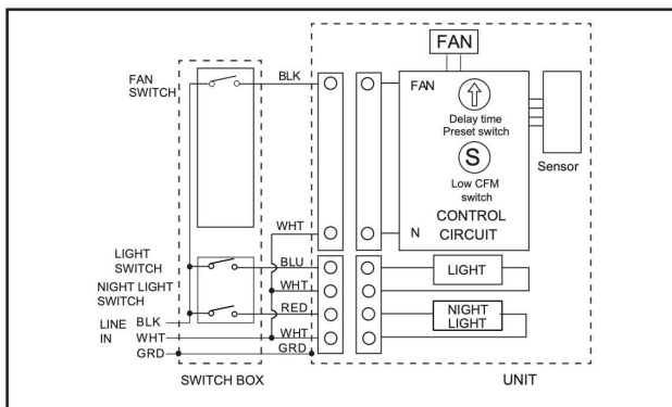
Fig.3 Fan with ADD on Motion Sensor Grille
