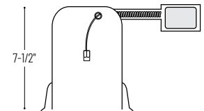
6-3/8" Ceiling Cut-out
