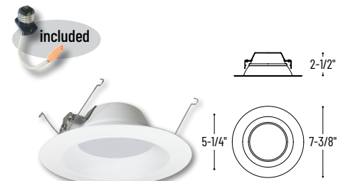
NOXAC-5631 Reflector
