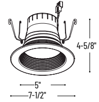
NLPR-5642 5 5/6" Baffle BZBZ, WW
