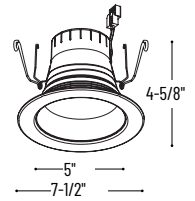
NLPR-5641 5 5/6" Reflector BB, BZBZ, HZW, WW
