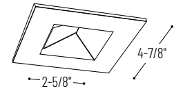
NIO-4SW Square Wall Wash Reflector Non-Adjustable
