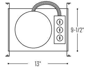
6-1/2" x 7" Ceiling Cut-out
