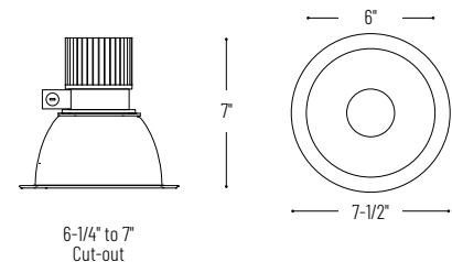
NCR-68 Decorative Glass Reflector (Specify glass separately)
