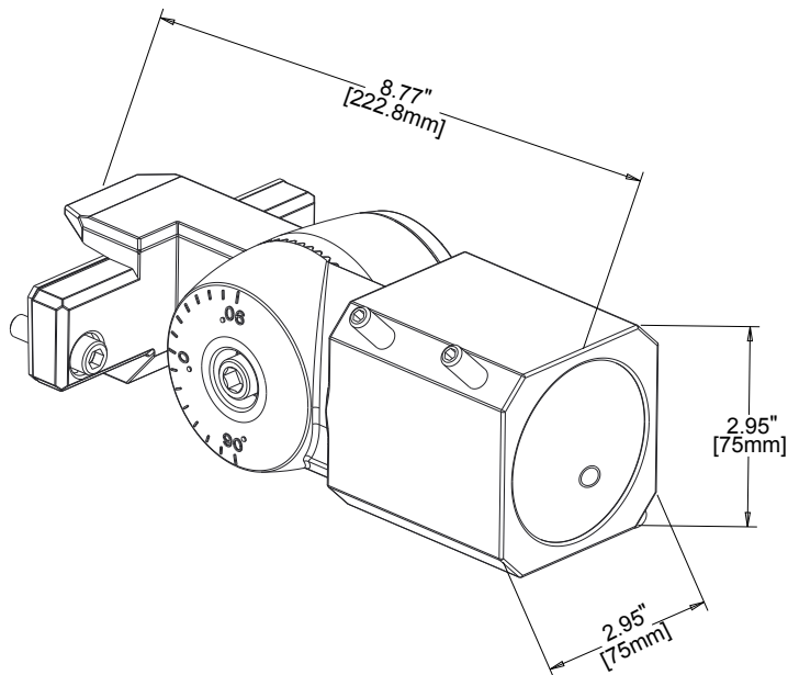
SLIPFITTER MOUNT QMP-SK
