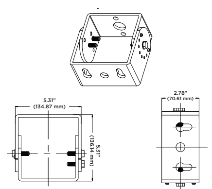
Trunnion Swivel
