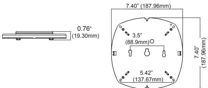
7"Round Light Engine
