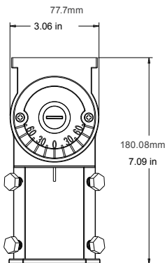
Slip Fitter Knuckle
