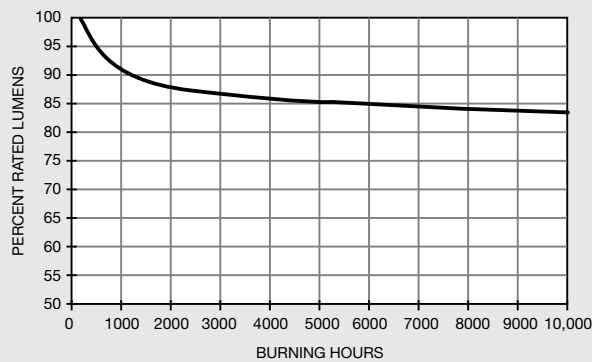
Lumen Maintenance Curve
