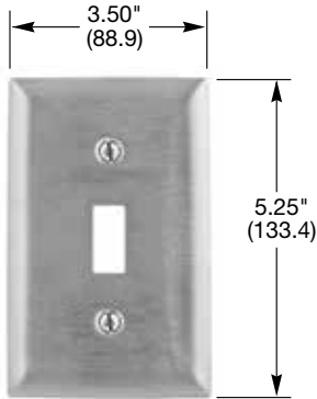
Jumbo Wallplate
