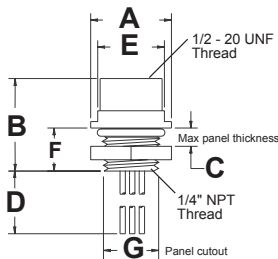
Female Inverse Receptacle 1/4" NPT Rear Thread
