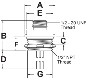
1/2" NPT Rear Thread Receptacle
