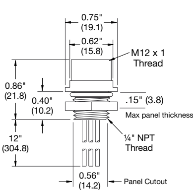
Female Inverse Receptacle Rear Thread - 1/4" NPT
