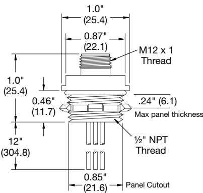
Male Receptacle Rear Thread - 1/2" NPT
