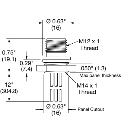
Male Receptacle Rear Thread - M14x1
