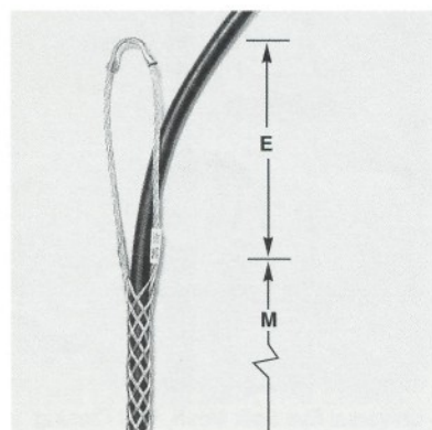
Heavy Duty, Single Eye, Closed Mesh
