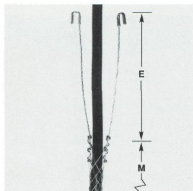
Hook End, Closed Mesh
