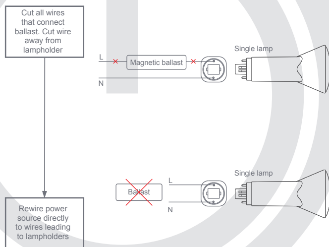
Diagram 2 – Magnetic ballast fixture wiring modification
