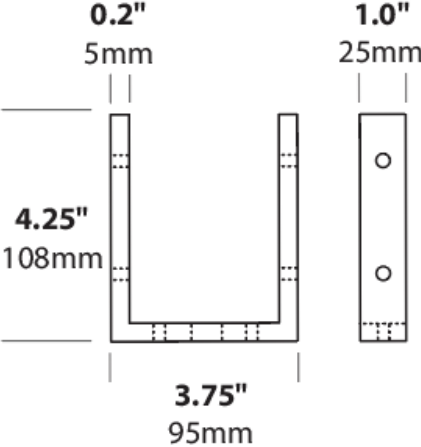
Steel U-Bracket Detail
