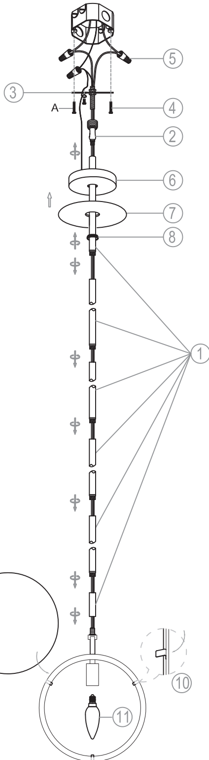
Wire connection
