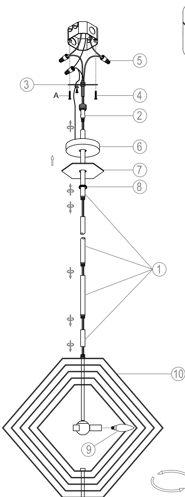
Wire connection
