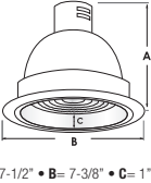
6114-CL Reflector with Frosted Glass Lens
