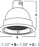
6115-WT Reflector with Tempered Clear Glass
