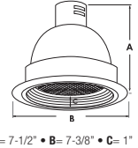
6113-WH Baffle with Tempered Clear Glass
