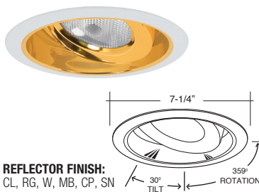
B1683RG-WH PAR36 REFLECTOR WITH GIMBAL RING
