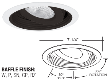
B1673P-WH PAR36 BAFFLE WITH GIMBAL RING
