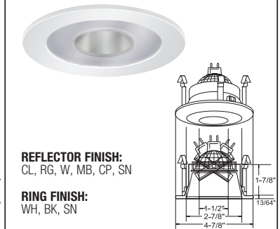
B1427CL-WH THE ILLUMINATOR
