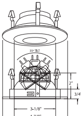
B1439WH SMOOTH FROST DOME SHOWER LITE
