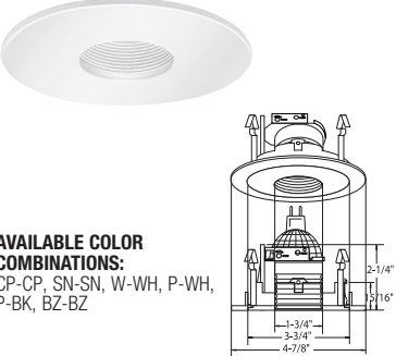
B1412CH FULLY ADJUSTABLE (35° TILT, 359° ROT.)
