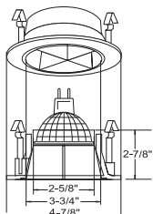
B1438WH DESIGNER POINT SHOWER LITE
