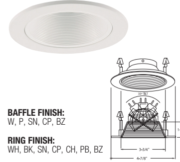
B1417W-WH METAL STEPPED BAFFLE
