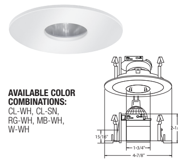
B1468W-WH FULLY ADJ. W/ BAFFLE (35° TILT, 359° ROT.)
