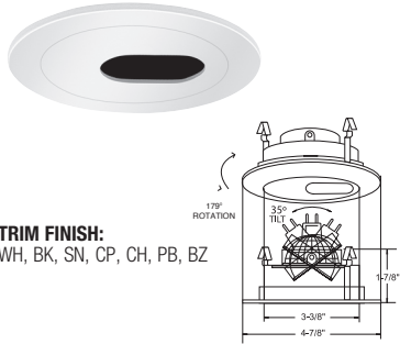
B1414W-WH PINHOLE WITH BAFFLE
