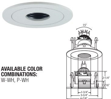
B1433P-WH ADJUSTABLE PINHOLE BAFFLE (15° TILT)
