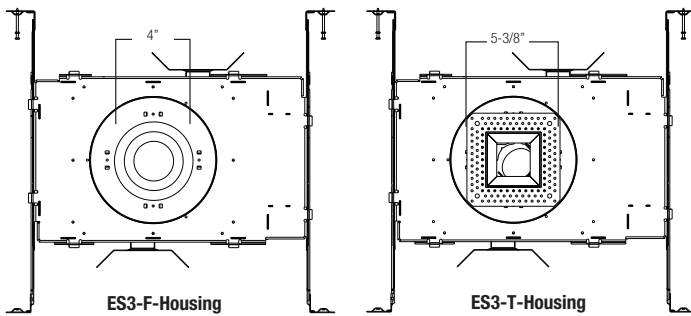
1302 - Lensed downlight
