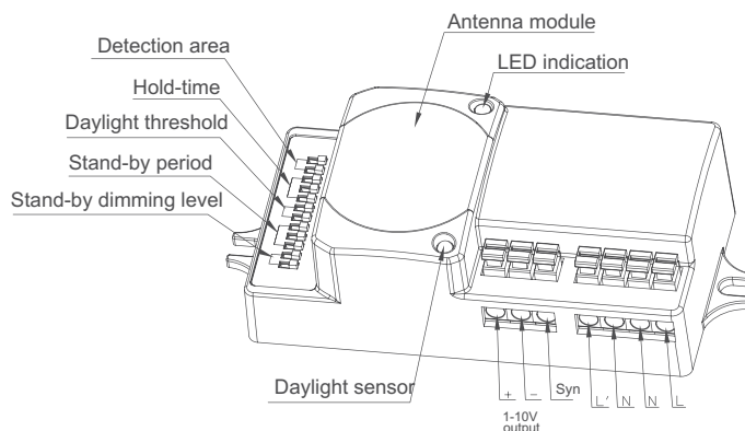
Tri-Level Dimming Sensor Control ULT-HC419V
