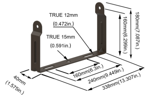
FOR 100W AL
