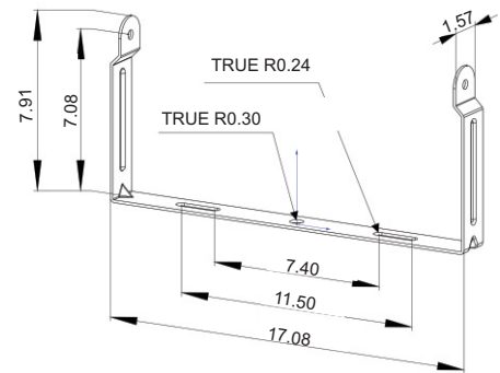
FOR 300W AL
