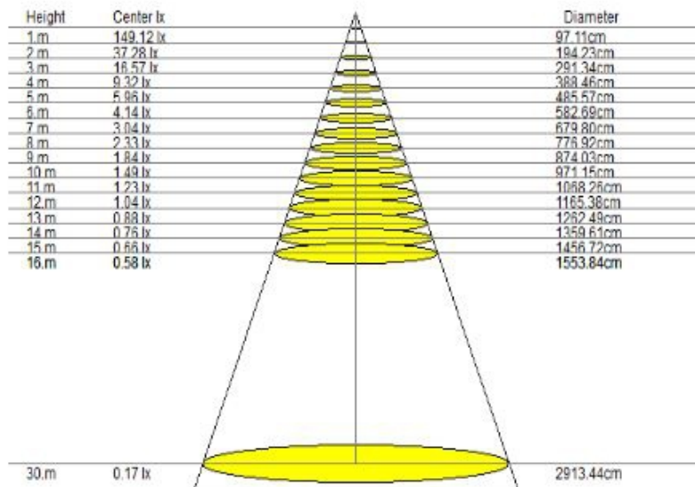
Light Distribution Curve Unit: cd
