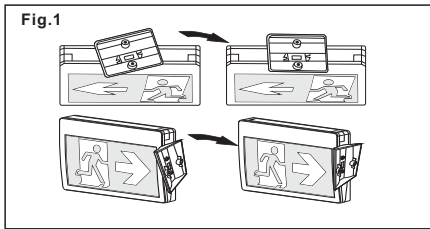
Canopy Assembly FIG #1&2
