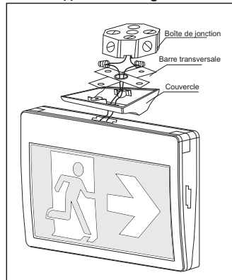
Support de mur Fig #7
