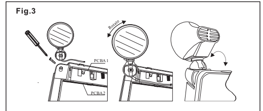
Assembly Lamp Heads (FIG 3)
