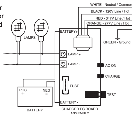
CHARGER BOARD STANDARD TRIPLE INPUT VERSION
