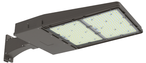
Hybrid Shoebox Flood Light (300W) with Wall-Mount SH-300W-50K-V4 + SH-WM-V4
