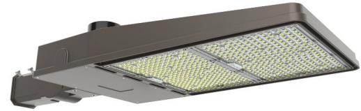
Hybrid Shoebox Flood Light (300W) with Slip-Fitter SH-300W-50K-V4 + SH-SL-V4
