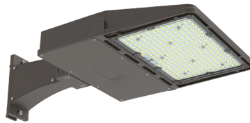
Hybrid Shoebox Flood Light (150W/200W) with Wall-Mount SH-150W-xxK-V4 + SH-WM-V4 SH-200W-xxK-V4 + SH-WM-V4
